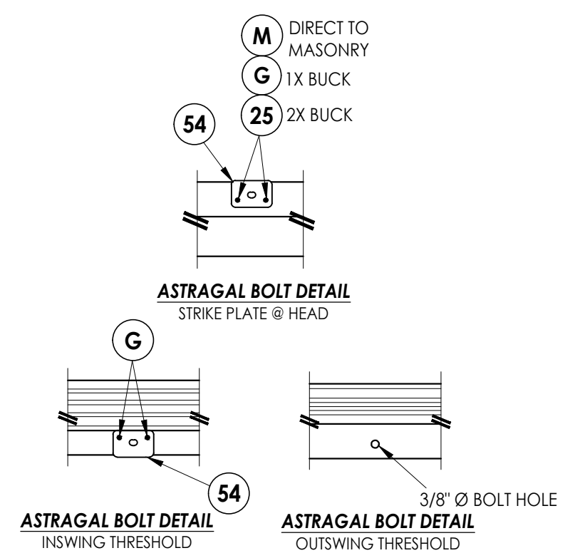
ASTRAGAL BOLT DETAIL INSWING THRESHOLD ASTRAGAL BOLT DETAIL OUTSWING THRESHOLD ASTRAGAL BOLT DETAIL STRIKE PLATE @ HEAD
