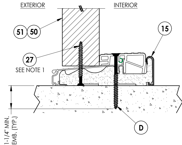
4 9 VERTICAL CROSS SECTION Outswing Sill
