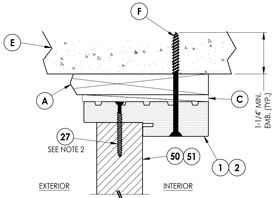
3 VERTICAL CROSS SECTION 7 Outswing Shown (Inswing Similar) Shown w/ 1X Buck
