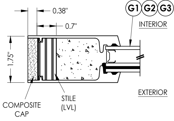
3 3 HORIZONTAL CROSS SECTION
